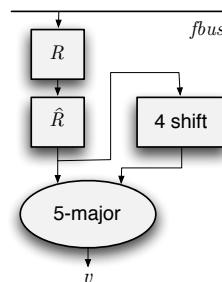
Fig. 8. Receiver Logic
