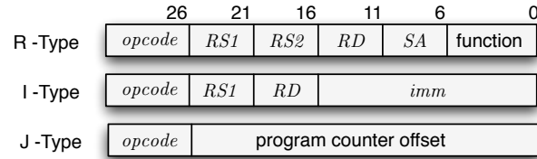
Fig. 13. Instruction Types
