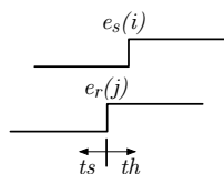
Fig. 5. Clock Edges
