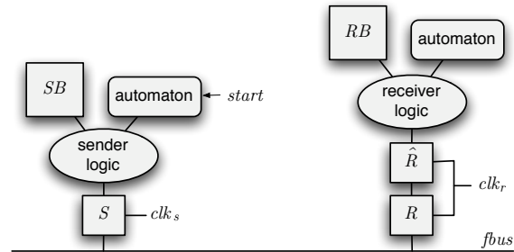
Fig. 7. Send and Receive Buffer
